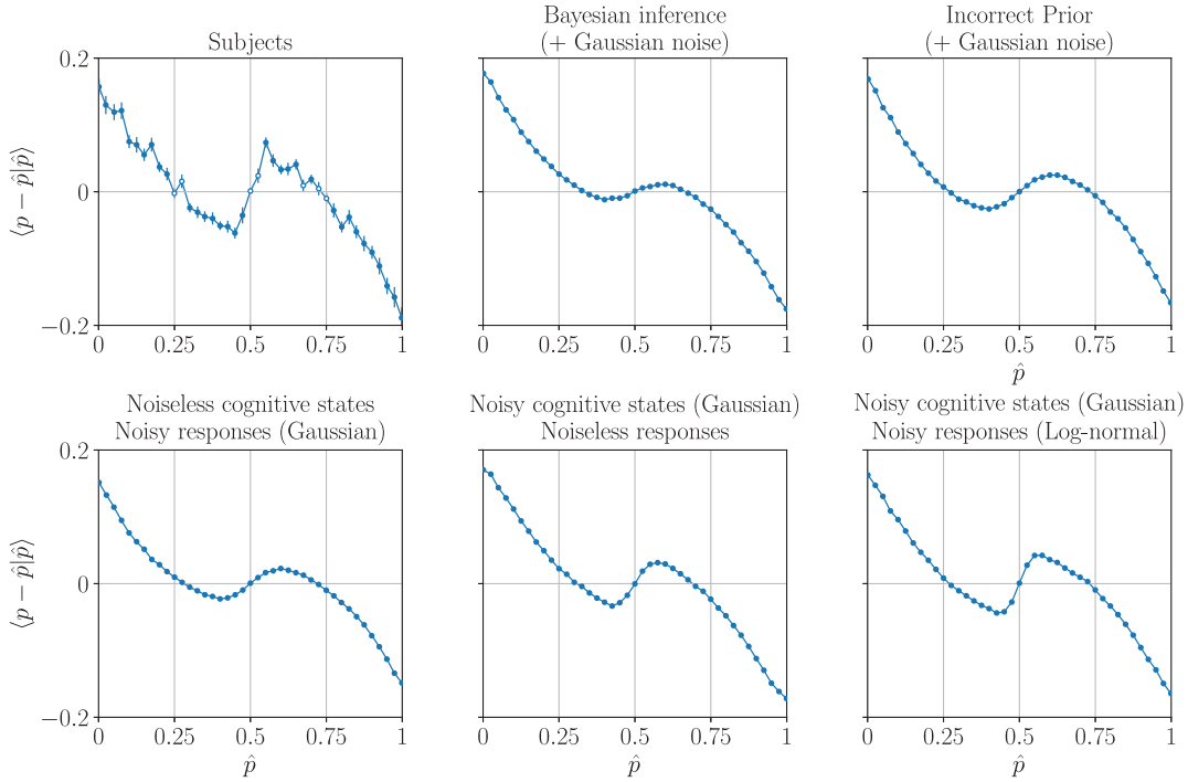
Figure 17 Subjects' and Model Subjects' Responses Do Not Verify the Calibrated-Response Property
