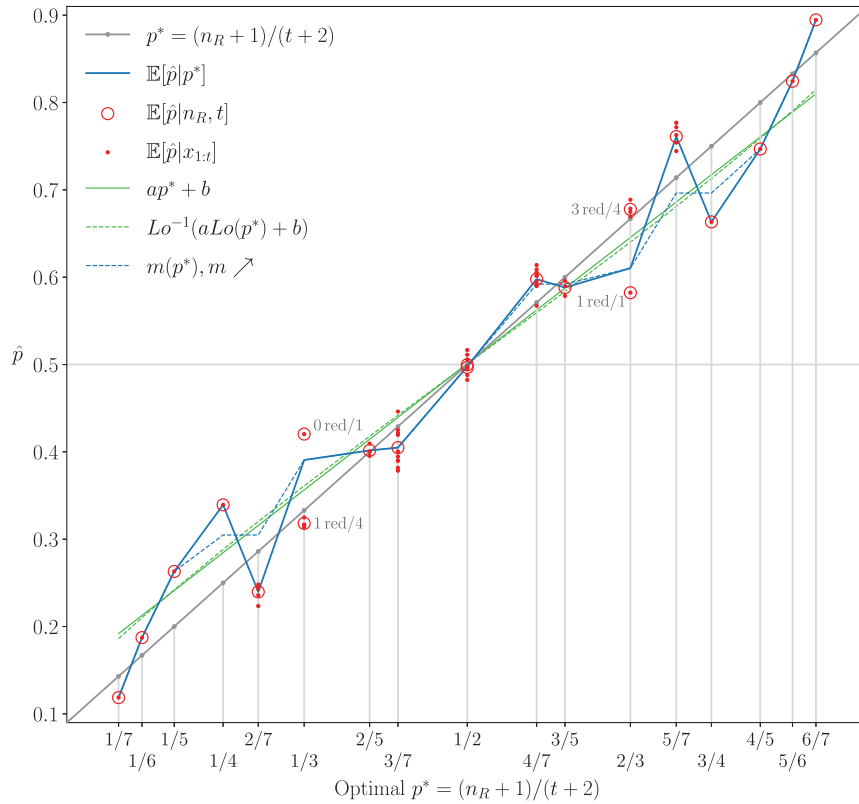
Figure 3 Subjects' Responses Are Poorly Captured by Functions of the Optimal Bayesian Estimate Alone
