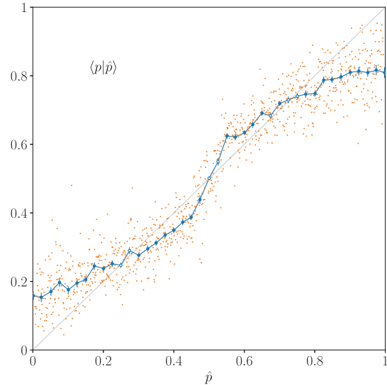
Figure 7 The Calibrated-Responses Bayesian Property Is Not Verified in Subjects' Responses
