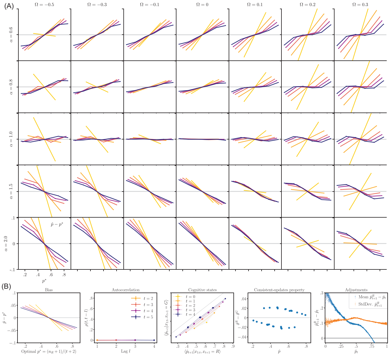
Note. (A) Bias of the model for different values of the parameters \alpha and \Omega . (B) Behavior of the best-fitting sequential-dependency model.
