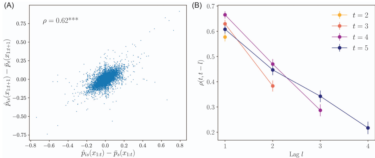
Figure 5 Autocorrelation in Subjects' Responses
