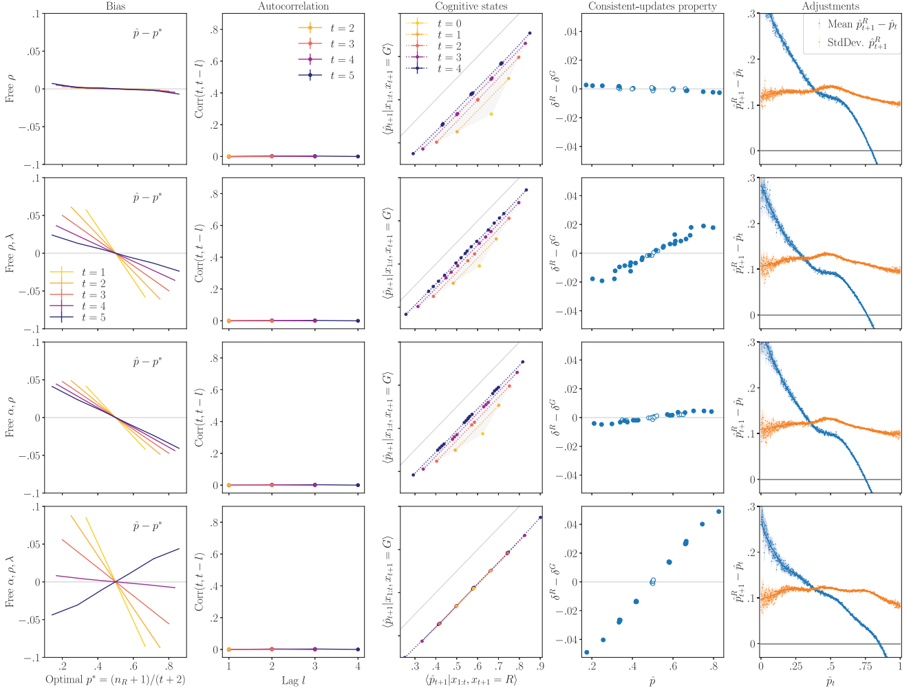
Figure 14 Behavior of the Quasi-Bayesian Models
